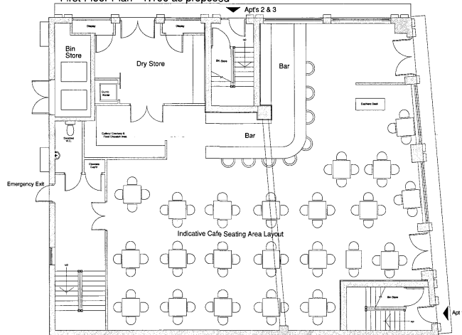
Ground Floor Plan - 1:100 as proposed
