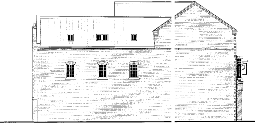
Side Elevation - 1:100 as proposed
